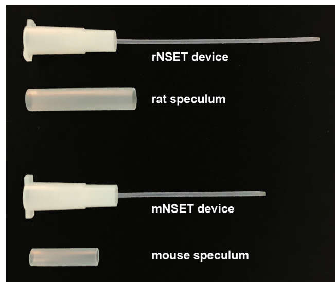
Figure 1. Manufactured rNSET device and speculum. The rNSET catheter is made from Teflon and the hub is molded from polyethylene. The hub is designed to fit securely on the end of a PR-2 pipette. The tip is tapered to facilitate passage through the cervix, with the length of the catheter (37 mm) optimized for embryo delivery through the cervix to the uterine horn. The catheter is flexible so that it readily passes through the cervix without damage to the uterine wall. The rat speculum is made from polyethylene and the length (19 mm) is optimized for use in SD and F344 rats. The mNSET and rNSET devices and specula are shown for comparison.
